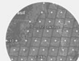
Mosaicos Landsat
